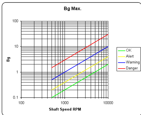
Fig.3. B_g Levels
